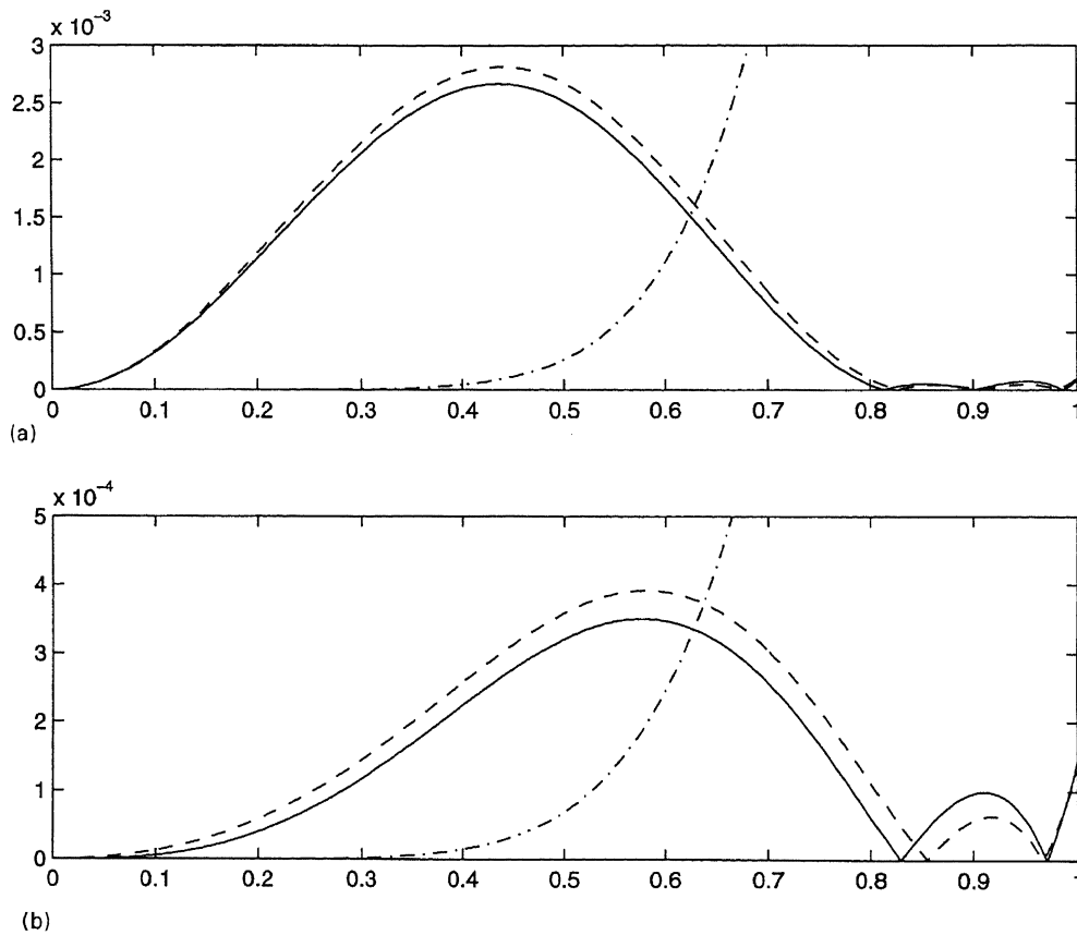
Fig. 2. (a) Plots of the max norm of (2.3) in [0,1] for OSC and SC (dash-dotted curve) methods. (b) Plots of the max norm of (2.3) on [0,1] for POSC and PSC (dash-dotted curve) methods.
